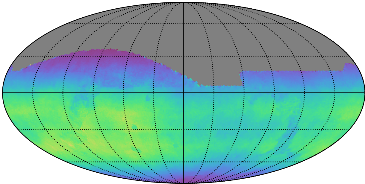
baseline_v3.2_10yrs All sky all bands: Normalized Teff
