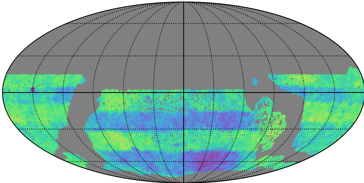
baseline_v3.2_10yrs WFD: Normalized Proper Motion Uncert @ 24.0
