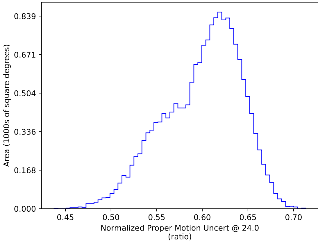
baseline_v3.2_10yrs WFD: Normalized Proper Motion Uncert @ 24.0
