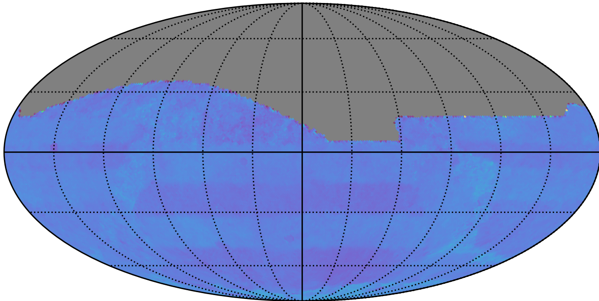
baseline_v3.2_10yrs All sky: Normalized Proper Motion Uncert @ 24.0
