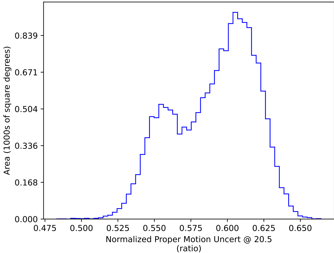
baseline_v3.2_10yrs WFD: Normalized Proper Motion Uncert @ 20.5
