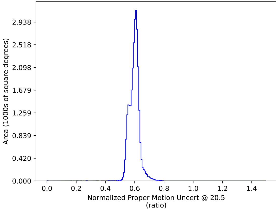
baseline_v3.2_10yrs All sky: Normalized Proper Motion Uncert @ 20.5
