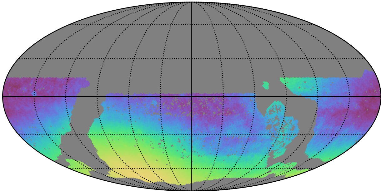
baseline_v3.2_10yrs WFD: Normalized Parallax Uncert @ 24.0
