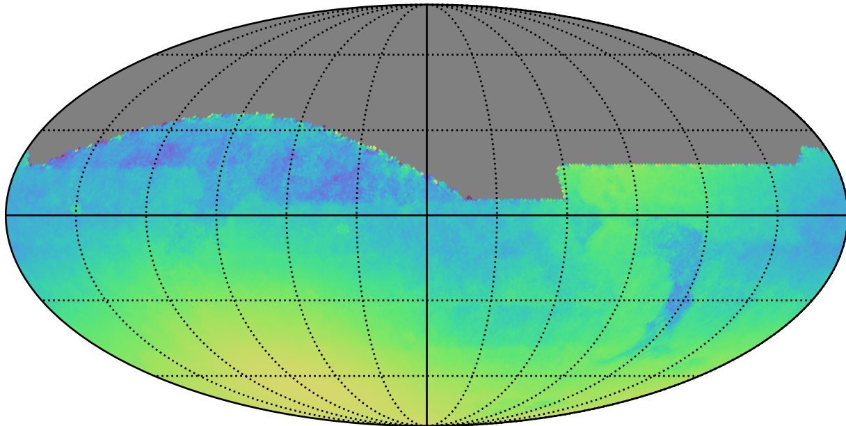
baseline_v3.2_10yrs All sky: Normalized Parallax Uncert @ 24.0
