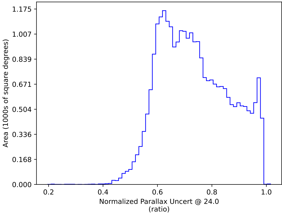
baseline_v3.2_10yrs All sky: Normalized Parallax Uncert @ 24.0
