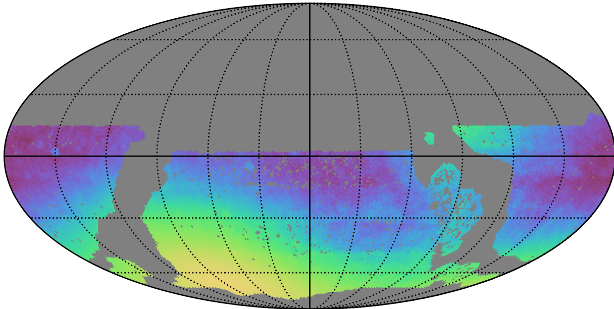
baseline_v3.2_10yrs WFD: Normalized Parallax Uncert @ 22.4
