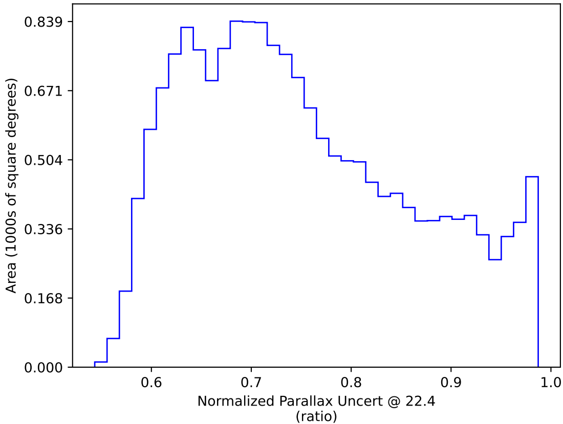
baseline_v3.2_10yrs WFD: Normalized Parallax Uncert @ 22.4
