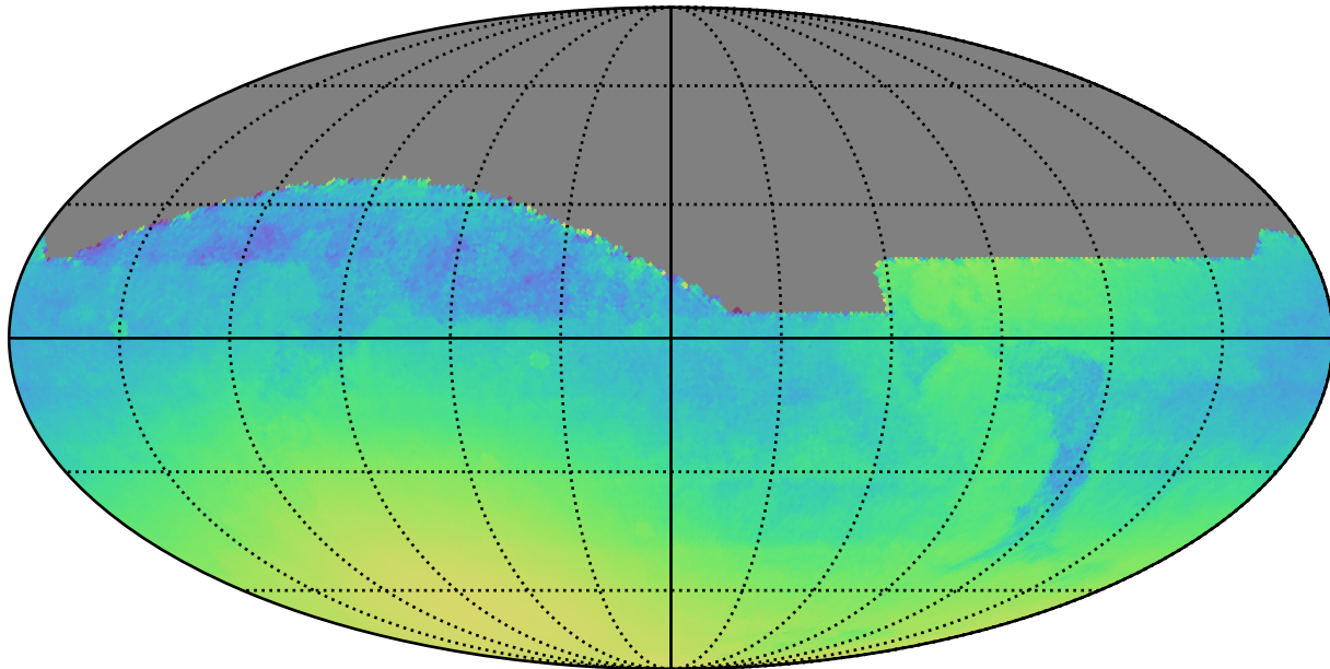
baseline_v3.2_10yrs All sky: Normalized Parallax Uncert @ 22.4
