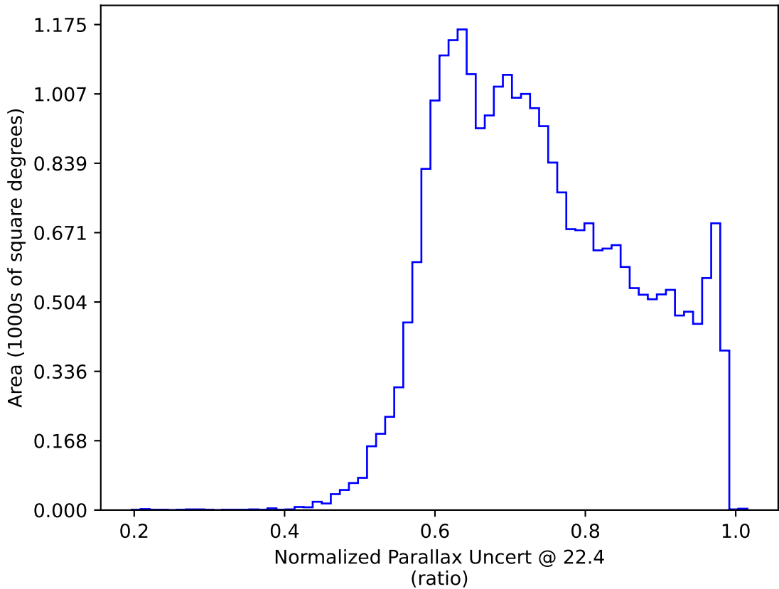
baseline_v3.2_10yrs All sky: Normalized Parallax Uncert @ 22.4
