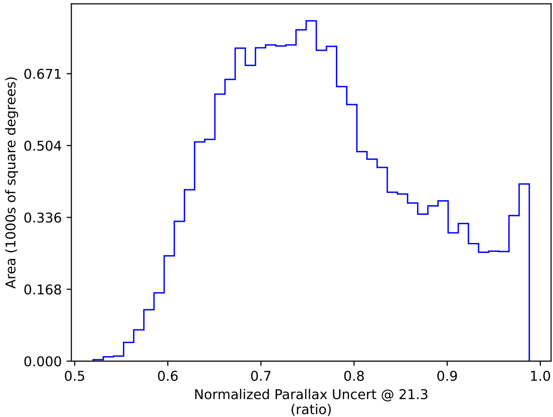
baseline_v3.2_10yrs WFD y band only: Normalized Parallax Uncert @ 21.3
