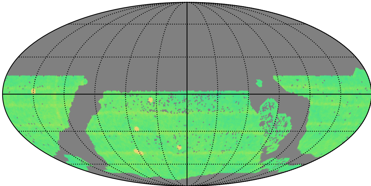
baseline_v3.2_10yrs WFD all bands: N Unique Nights
