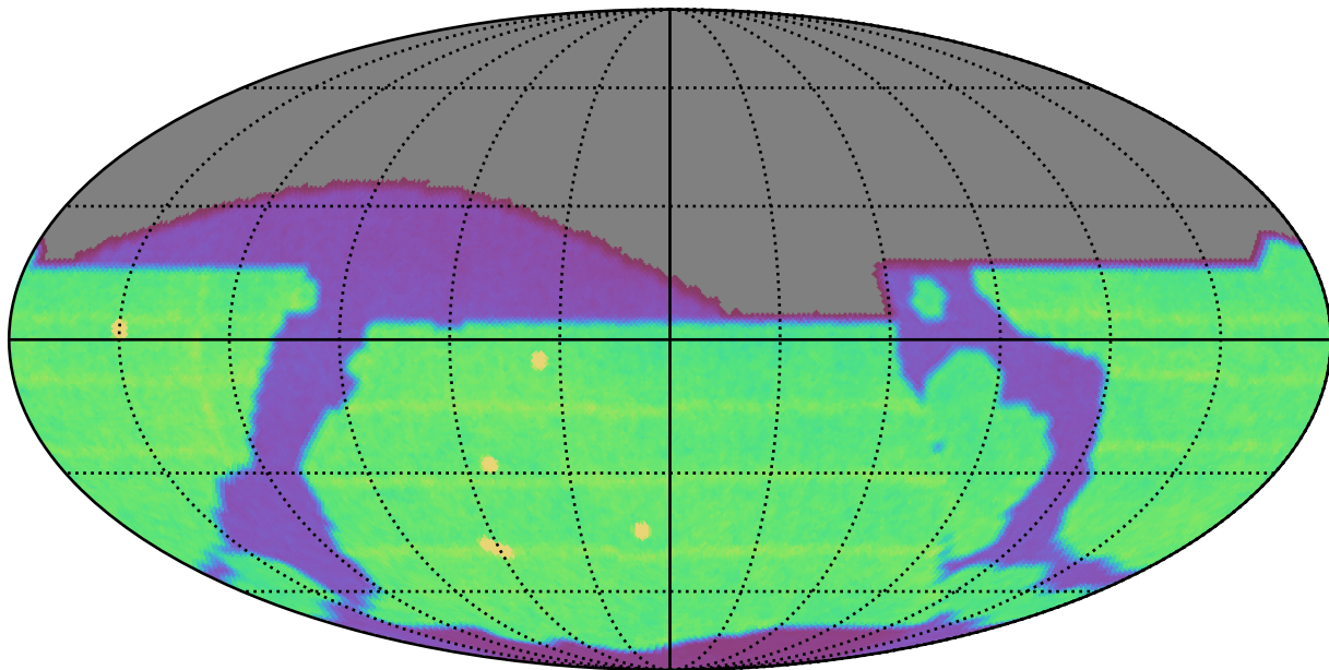
baseline_v3.2_10yrs All sky all bands: N Unique Nights
