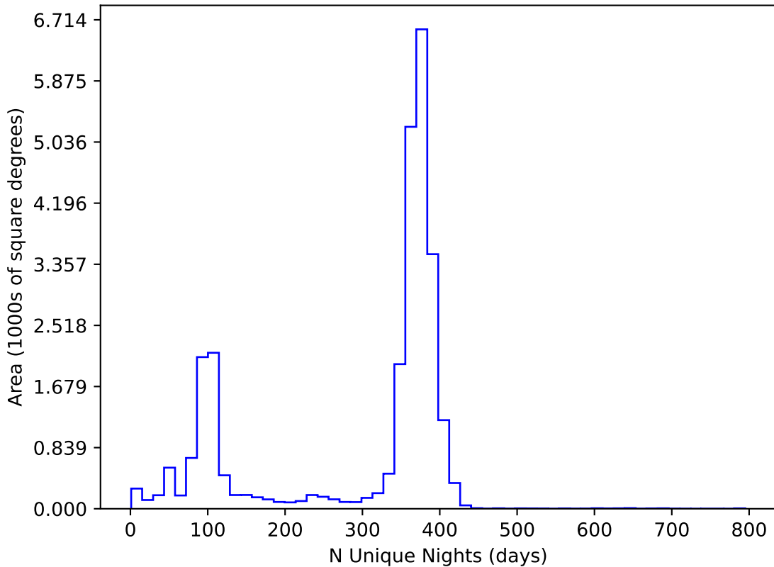
baseline_v3.2_10yrs All sky all bands: N Unique Nights
