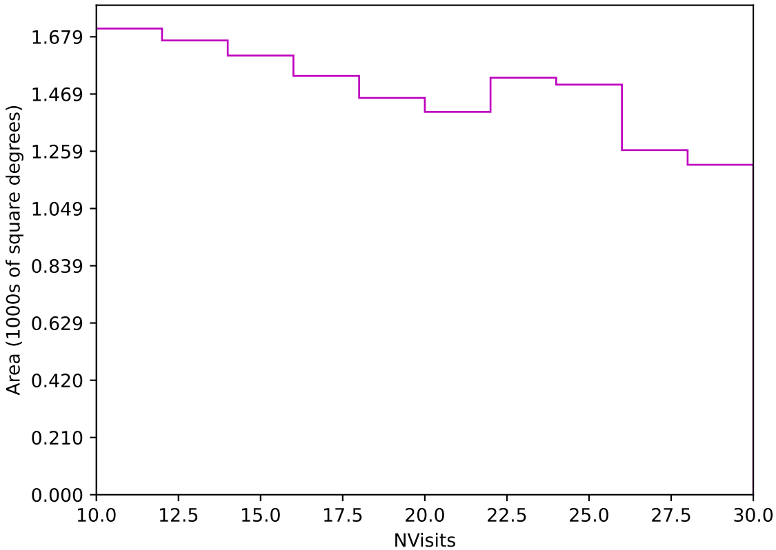
baseline_v3.2_10yrs Yr 3-4 z band: NVisits
