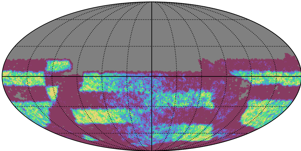
baseline_v3.2_10yrs Yr 3-4 y band: NVisits
