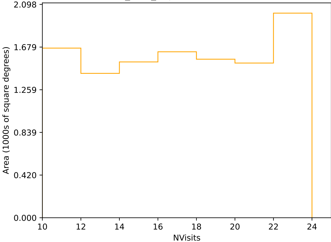
baseline_v3.2_10yrs Yr 3-4 r band: NVisits
