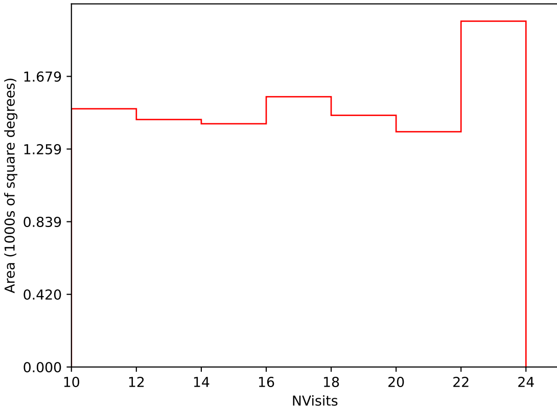
baseline_v3.2_10yrs Yr 3-4 i band: NVisits
