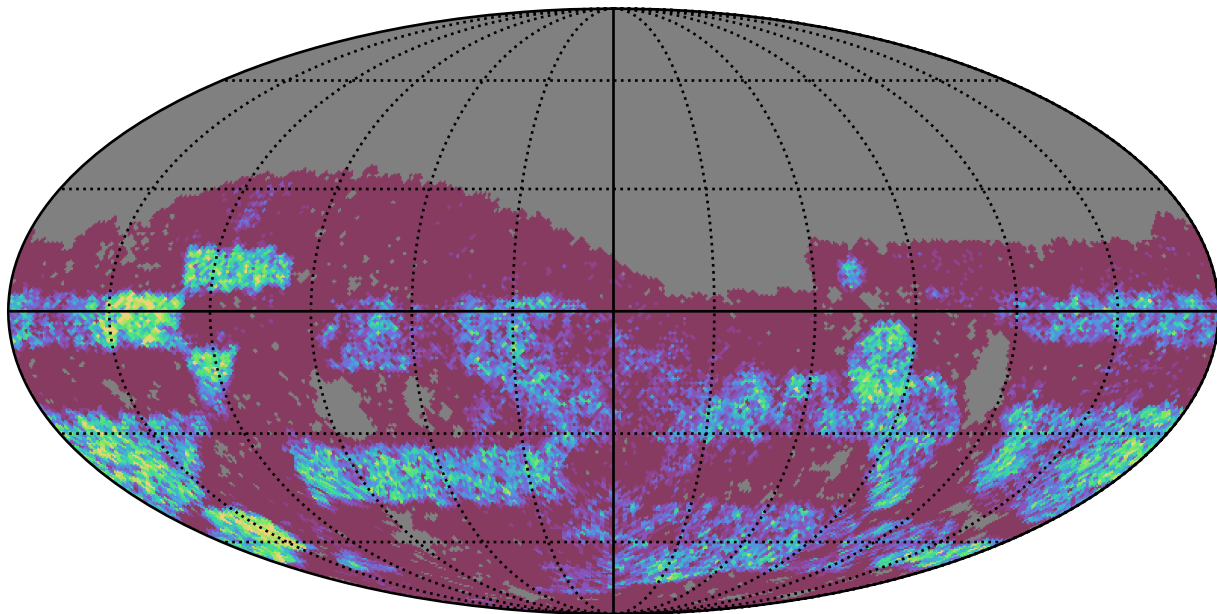
baseline_v3.2_10yrs Yr 3-4 g band: NVisits
