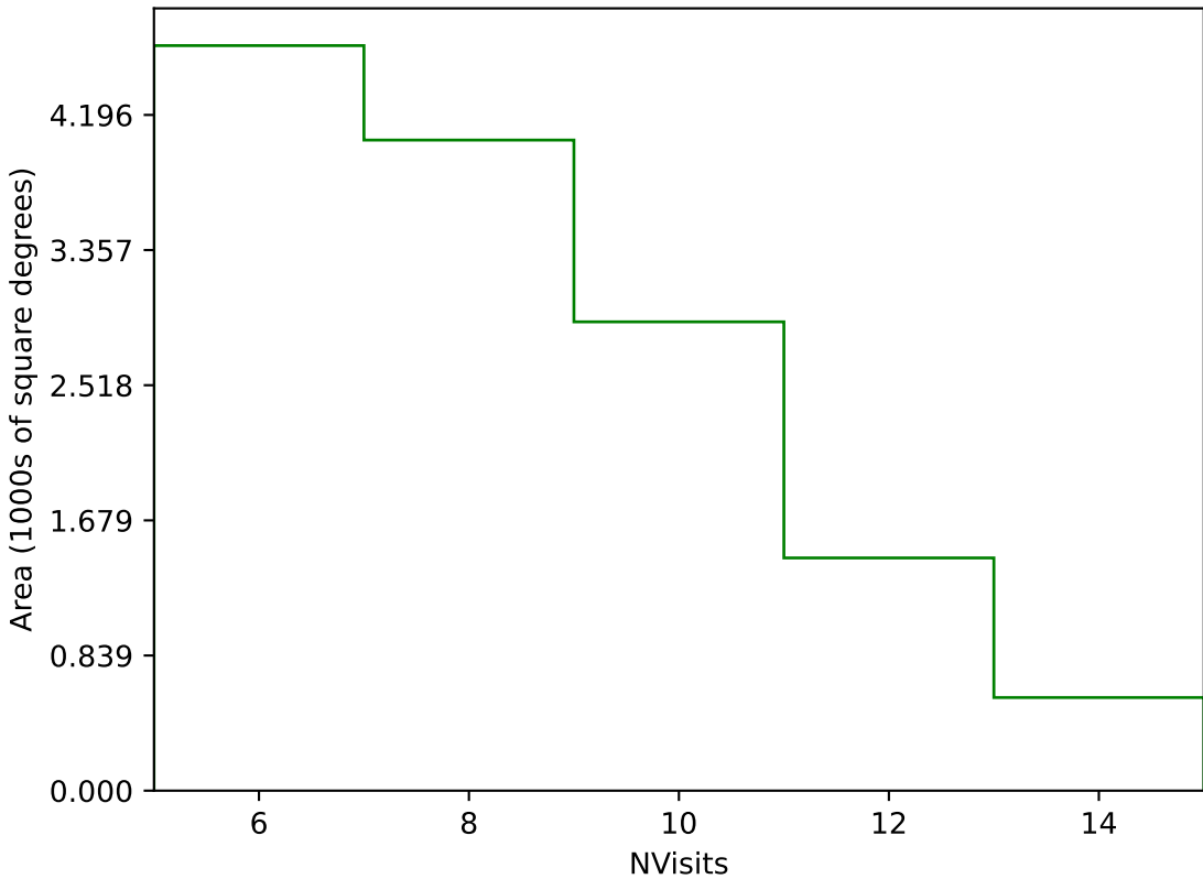
baseline_v3.2_10yrs Yr 3-4 g band: NVisits
