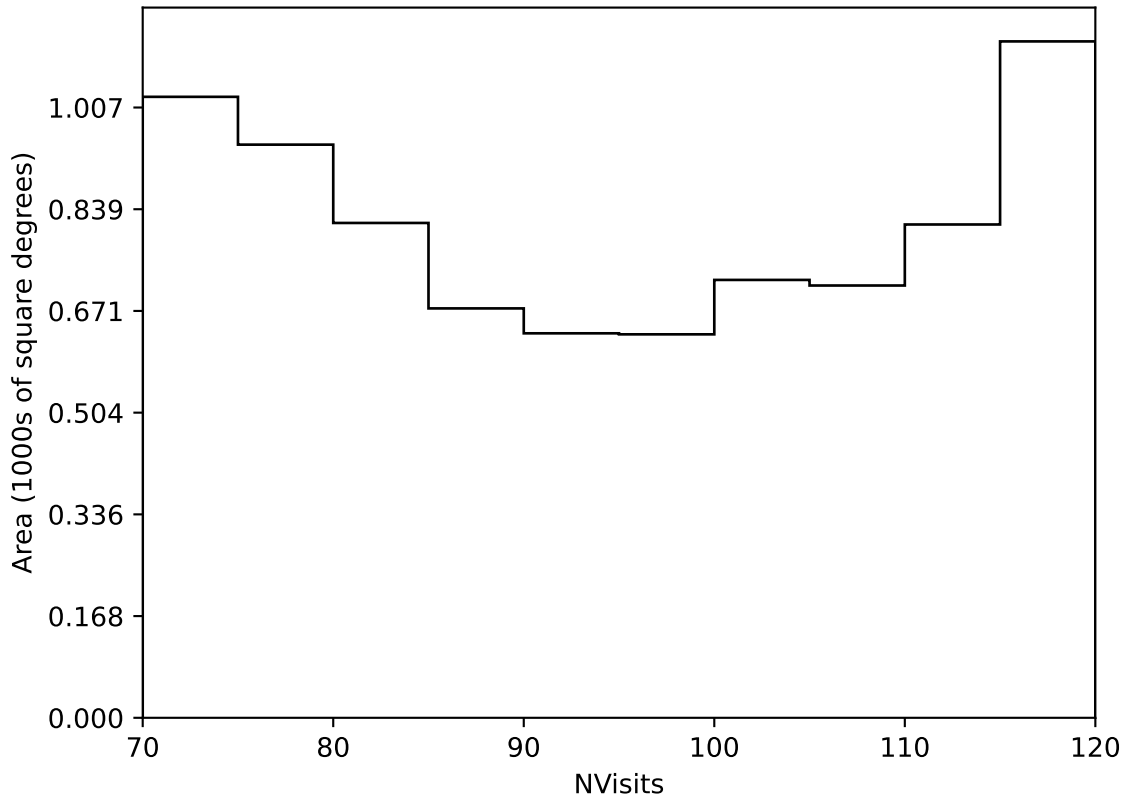
baseline_v3.2_10yrs Yr 3-4 all bands: NVisits
