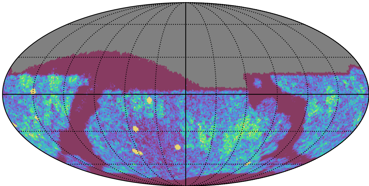
baseline_v3.2_10yrs Yr 1 z band: NVisits
