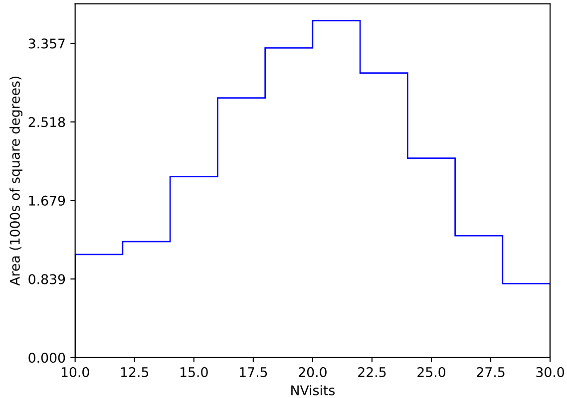
baseline_v3.2_10yrs Yr 1 y band: NVisits
