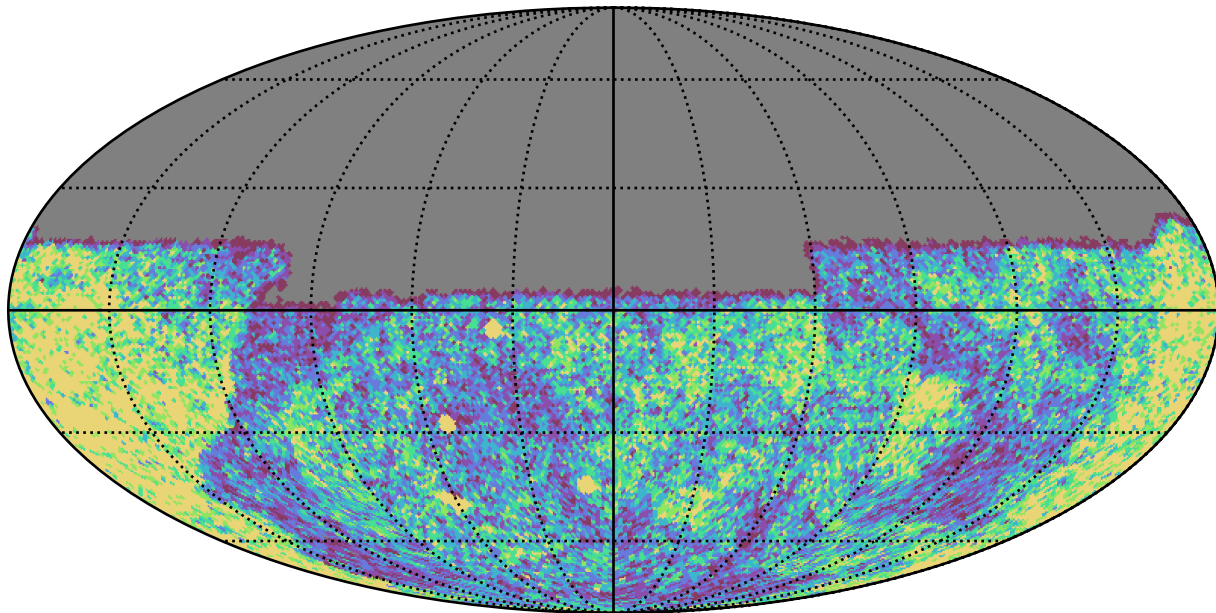
baseline_v3.2_10yrs Yr 1 u band: NVisits
