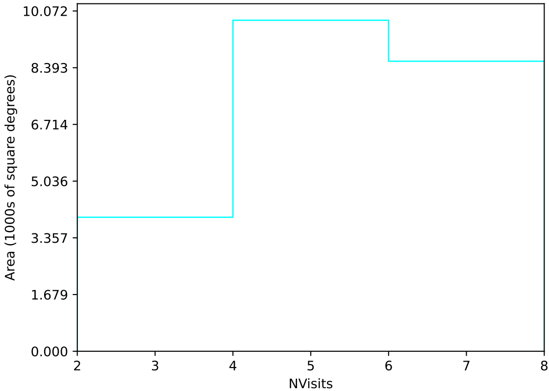
baseline_v3.2_10yrs Yr 1 u band: NVisits
