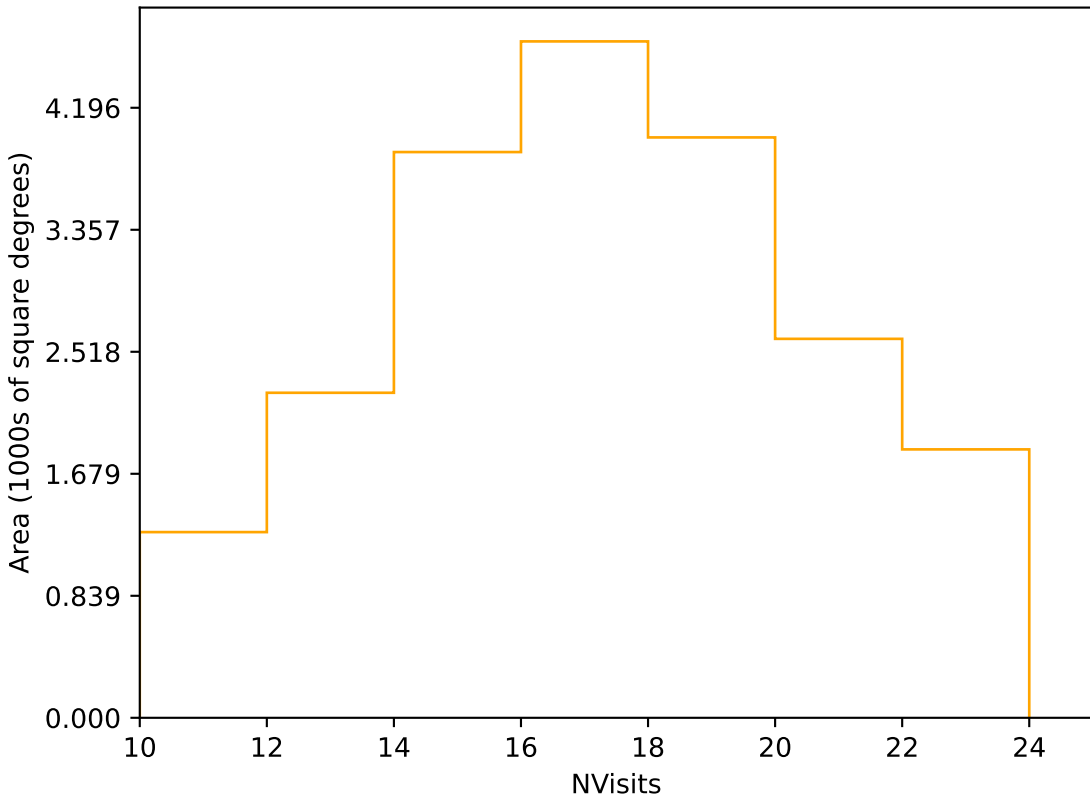
baseline_v3.2_10yrs Yr 1 r band: NVisits
