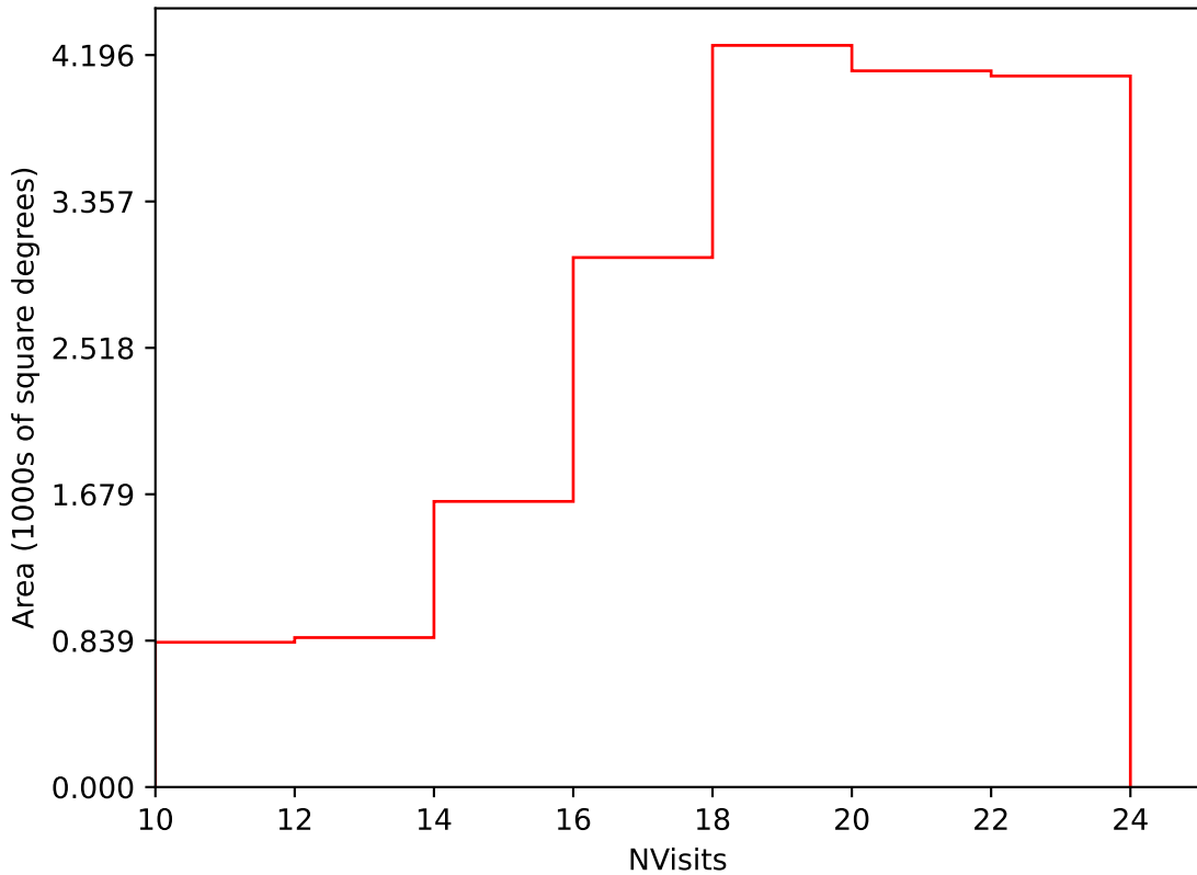
baseline_v3.2_10yrs Yr 1 i band: NVisits
