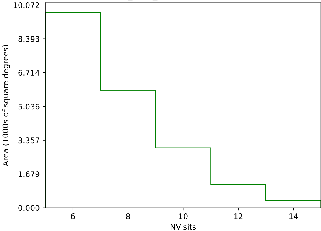
baseline_v3.2_10yrs Yr 1 g band: NVisits
