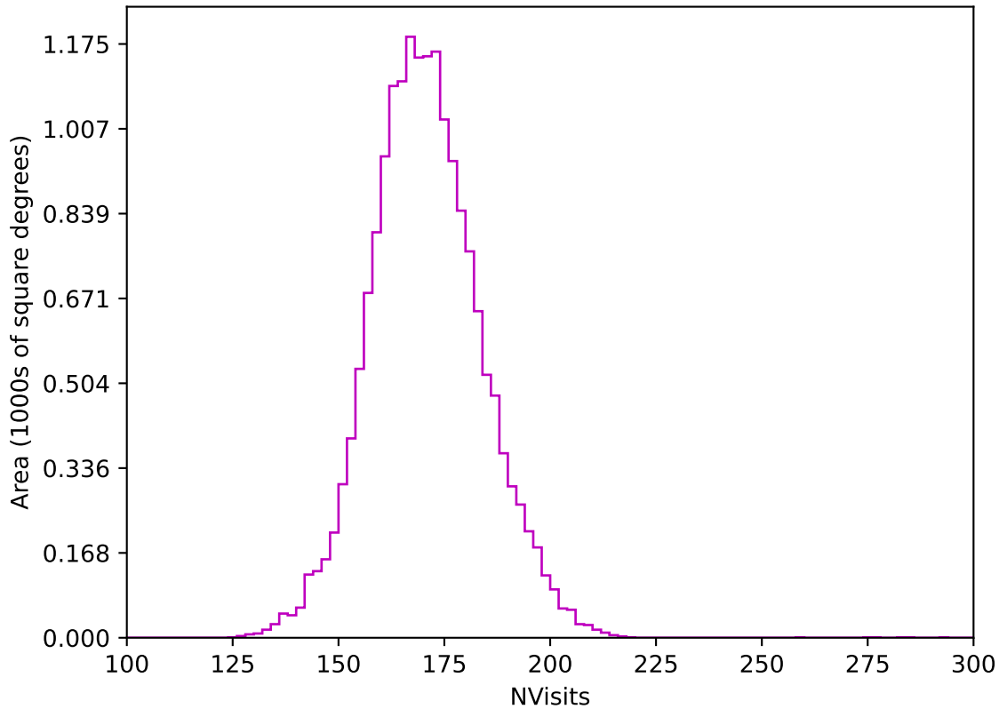
baseline_v3.2_10yrs WFD z band: NVisits
