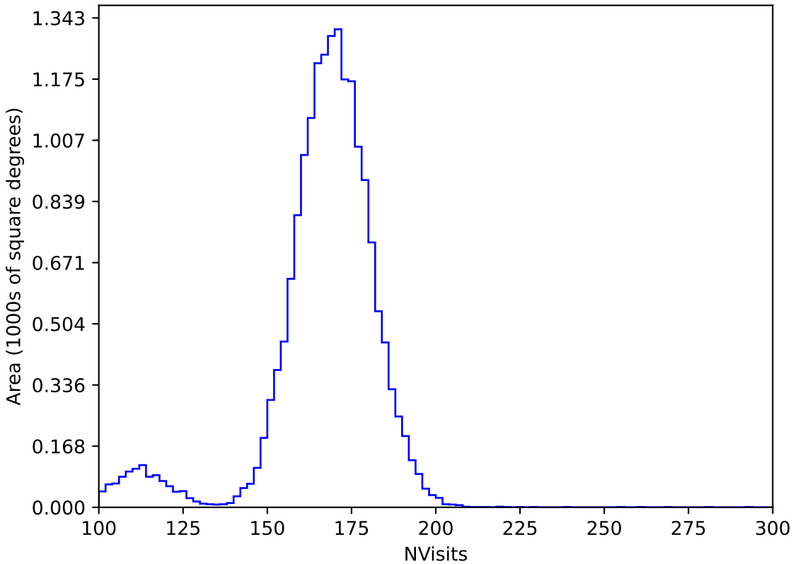
baseline_v3.2_10yrs WFD y band: NVisits
