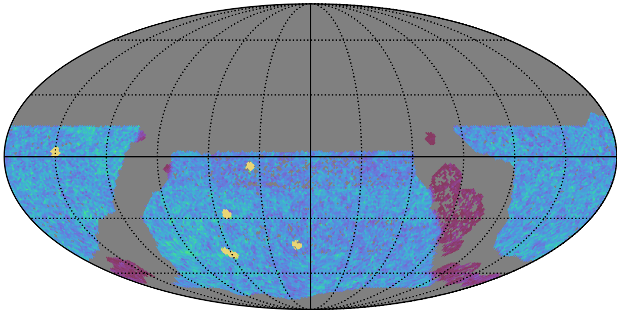
baseline_v3.2_10yrs WFD u band: NVisits
