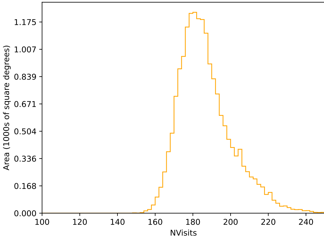
baseline_v3.2_10yrs WFD r band: NVisits
