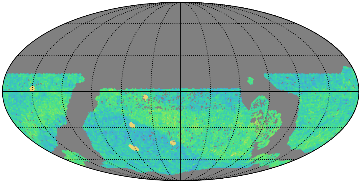
baseline_v3.2_10yrs WFD i band: NVisits
