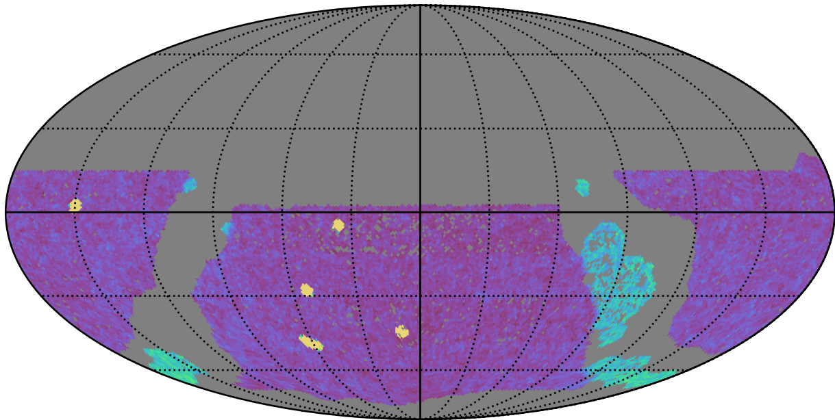
baseline_v3.2_10yrs WFD g band: NVisits
