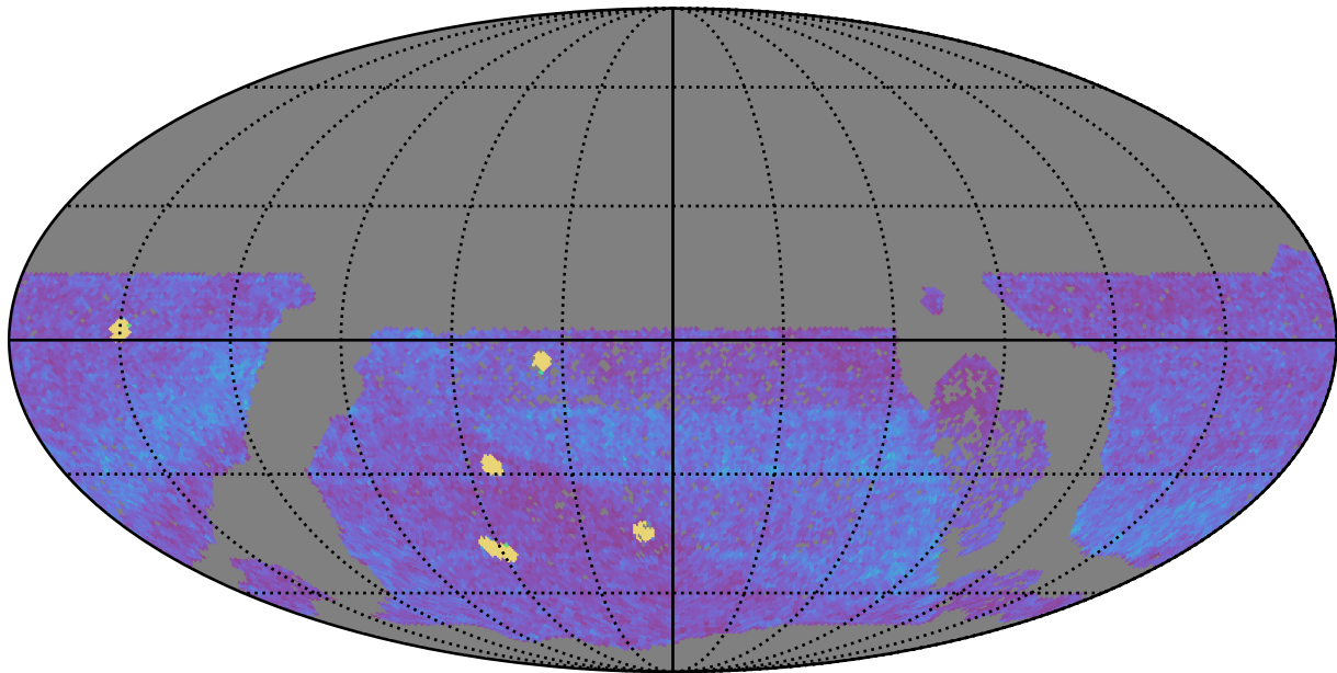
baseline_v3.2_10yrs WFD all bands: NVisits
