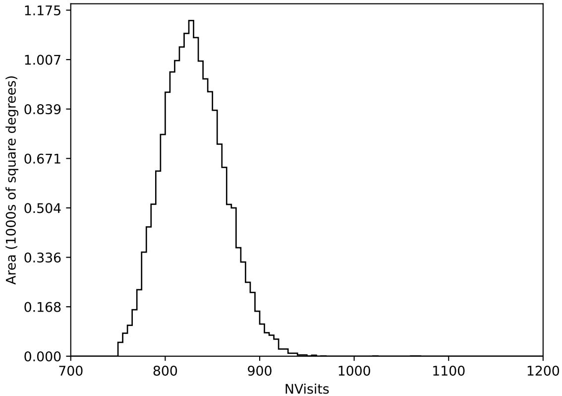
baseline_v3.2_10yrs WFD all bands: NVisits
