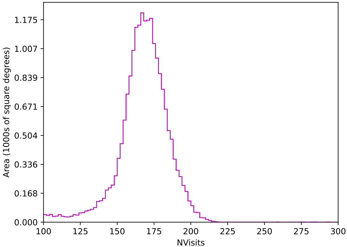
baseline_v3.2_10yrs All sky z band: NVisits
