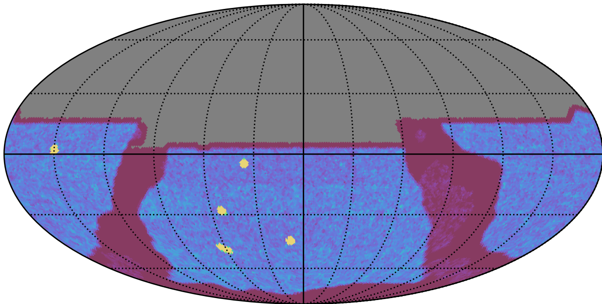
baseline_v3.2_10yrs All sky y band: NVisits
