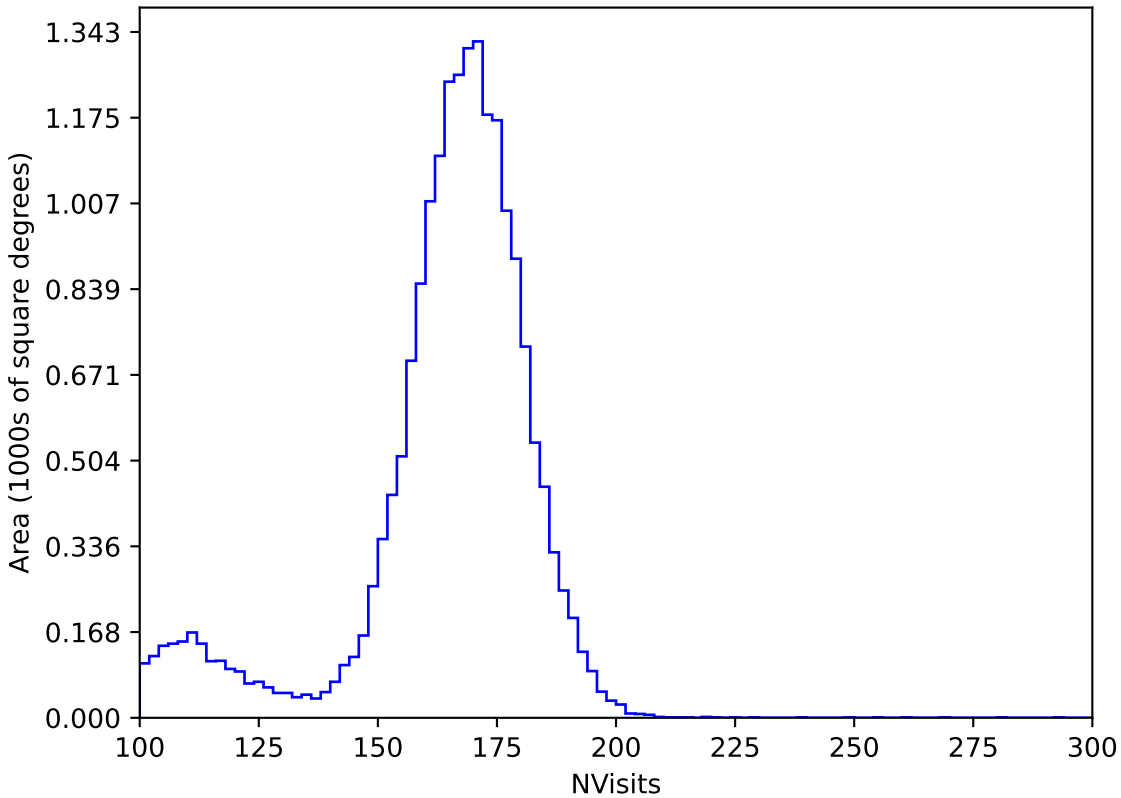
baseline_v3.2_10yrs All sky y band: NVisits
