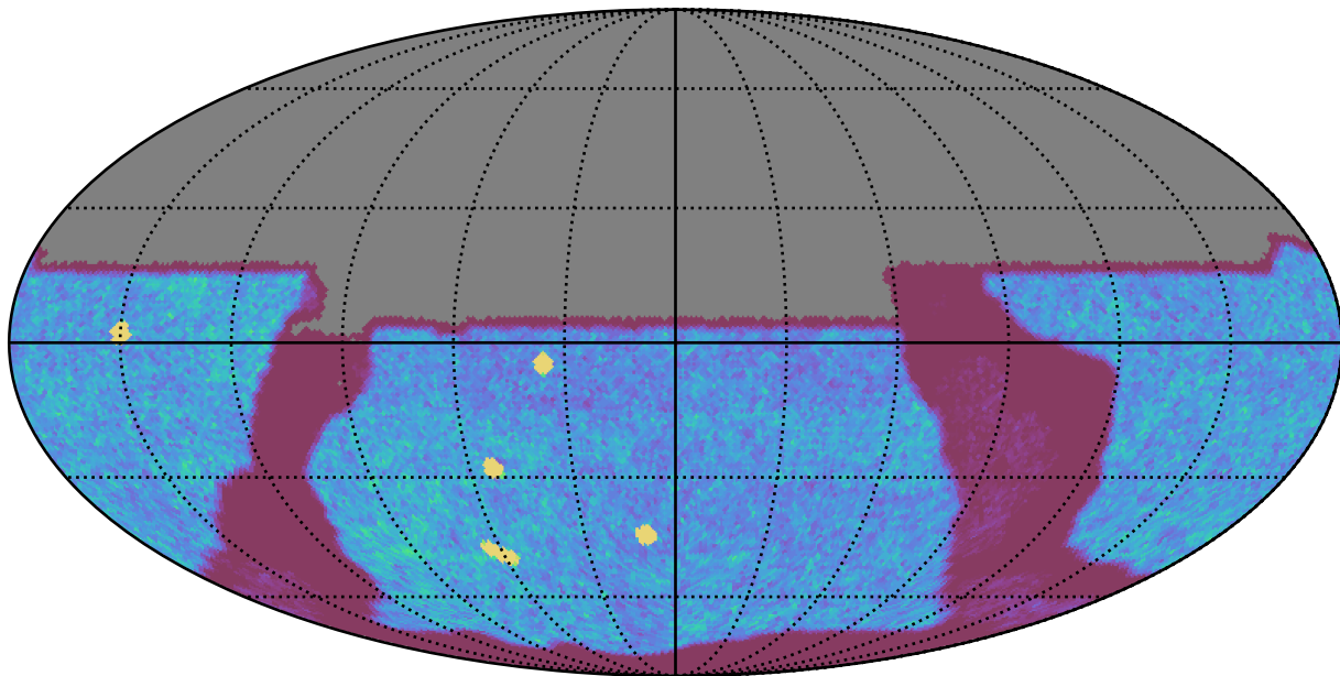
baseline_v3.2_10yrs All sky u band: NVisits
