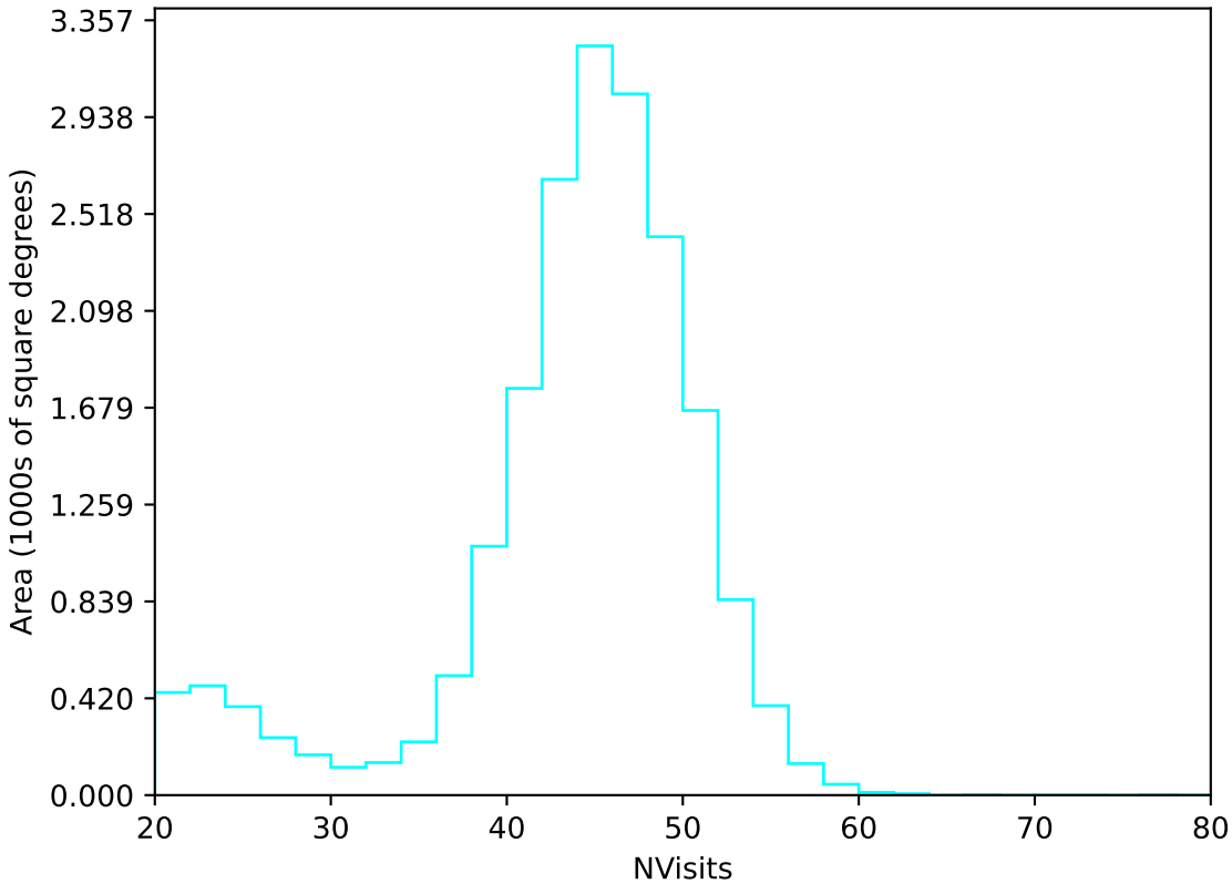
baseline_v3.2_10yrs All sky u band: NVisits
