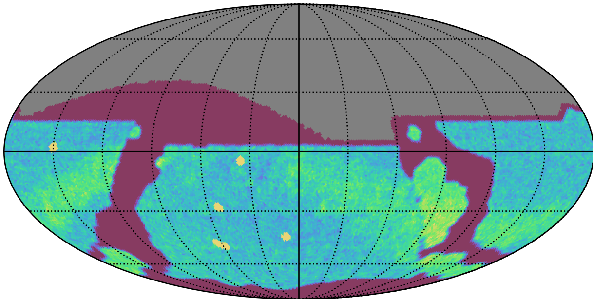
baseline_v3.2_10yrs All sky r band: NVisits
