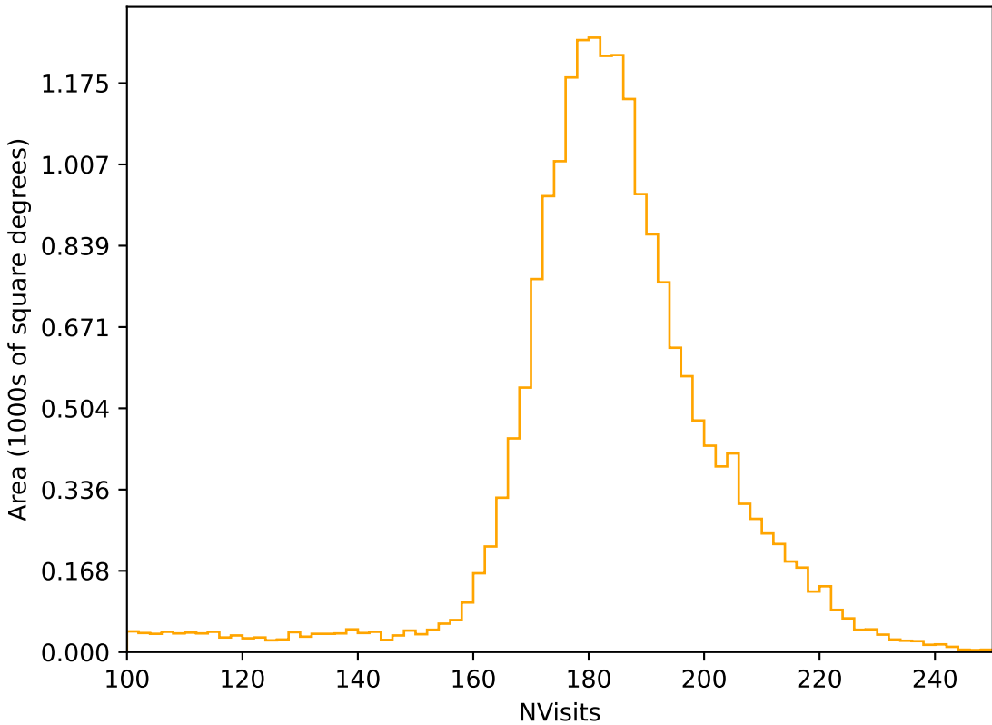
baseline_v3.2_10yrs All sky r band: NVisits
