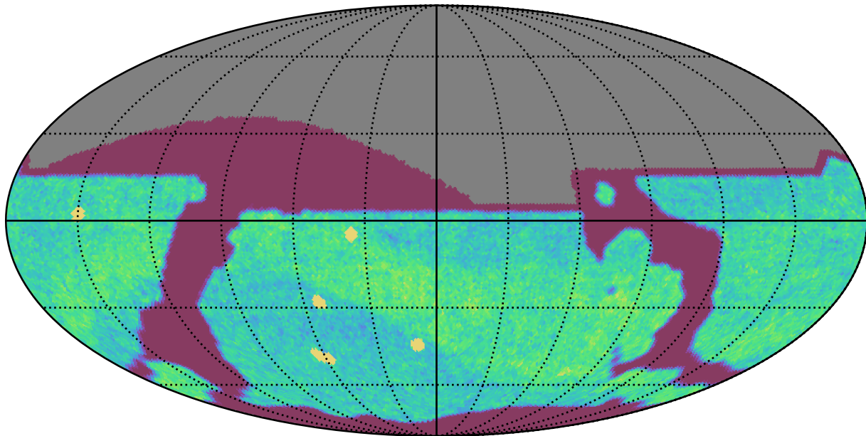
baseline_v3.2_10yrs All sky i band: NVisits
