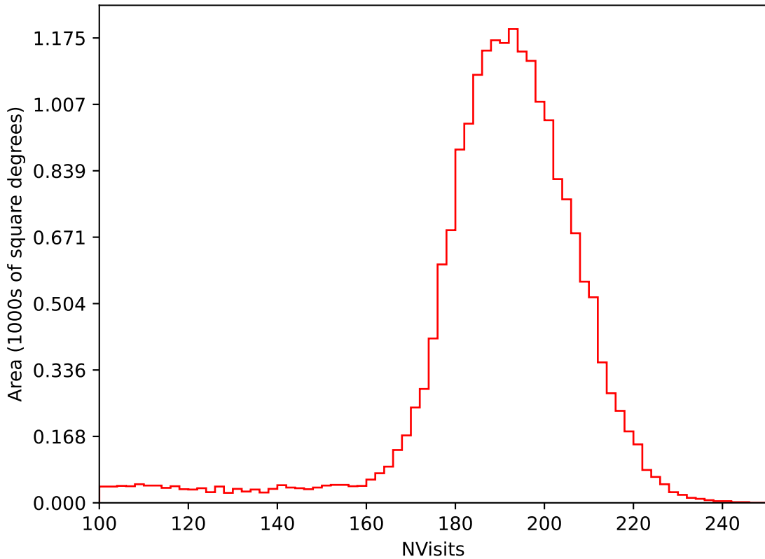
baseline_v3.2_10yrs All sky i band: NVisits
