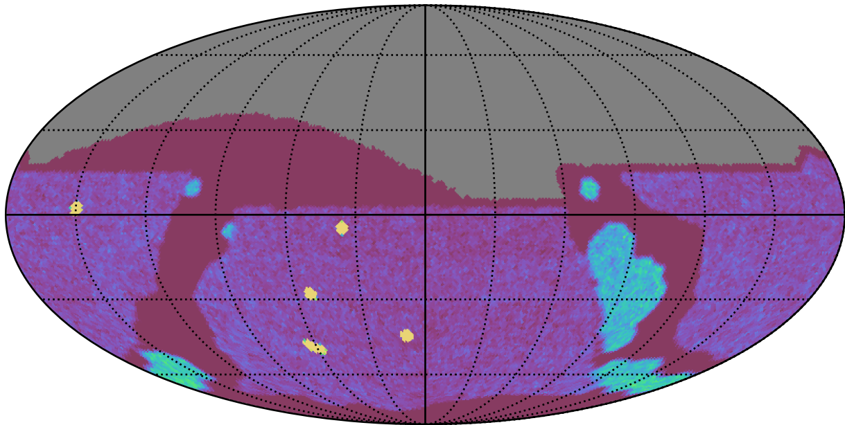
baseline_v3.2_10yrs All sky g band: NVisits
