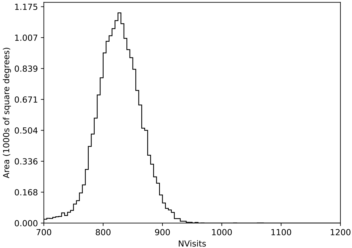
baseline_v3.2_10yrs All sky all bands: NVisits
